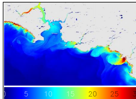
Figure 3: Landsat-8 OLI image of the Plymouth area 4 Nov 2013 showing suspended particulate concentration (mg/L).
